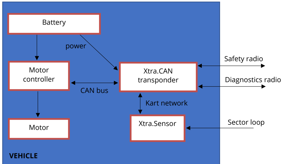
Figure 7 – Typical go-kart configuration
